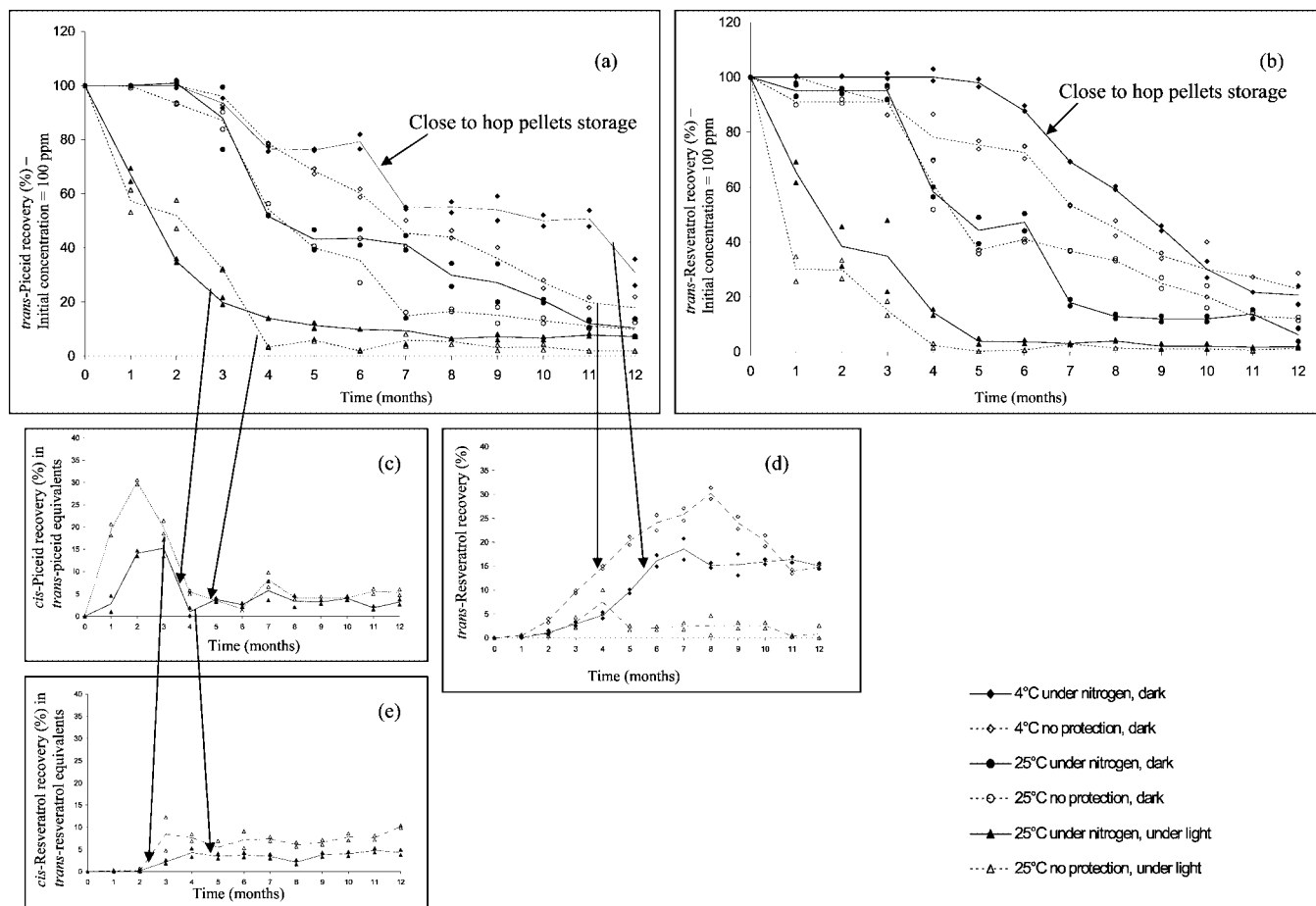
Figure 4. Evolution of stilbenes in aqueous solutions under various conditions. (a) Model medium spiked with trans -piceid, (b) model medium spiked with trans -resveratrol, (c) cis -piceid, (d) trans -resveratrol, and (e) cis -resveratrol formation in the trans -piceid spiked media stored under light (c and e) or in the dark (d).
